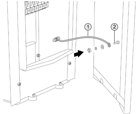
Abb. 9: Frontplatte erden
